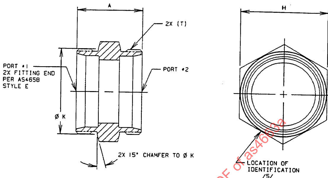
FIGURE 1 - FITTING, UNION, SHORT FLARELESS
