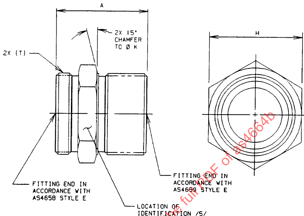
FIGURE 1 – FITTING, UNION, BULKHEAD, SHORT FLARELESS
