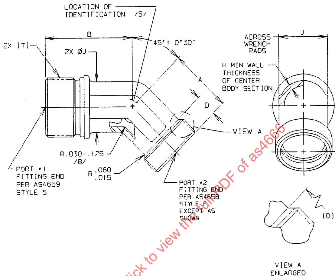
FIGURE 1 - ELBOW, 45°
