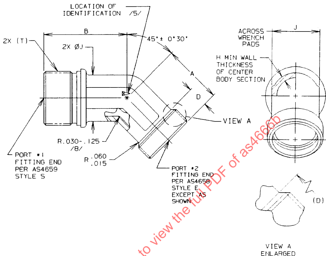
FIGURE 1 - FITTING, ELBOW, 45°
