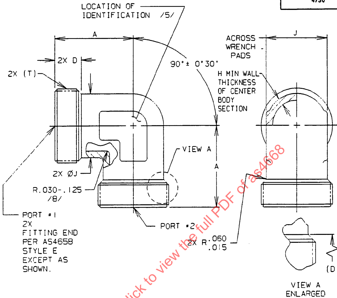
FIGURE 1 - ELBOW, 90°
