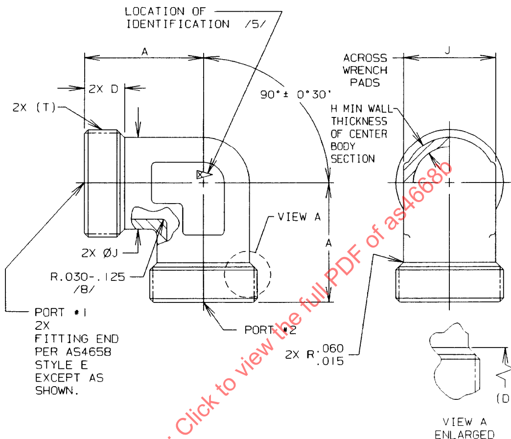
FIGURE 1 - FITTING, ELBOW, 90°
