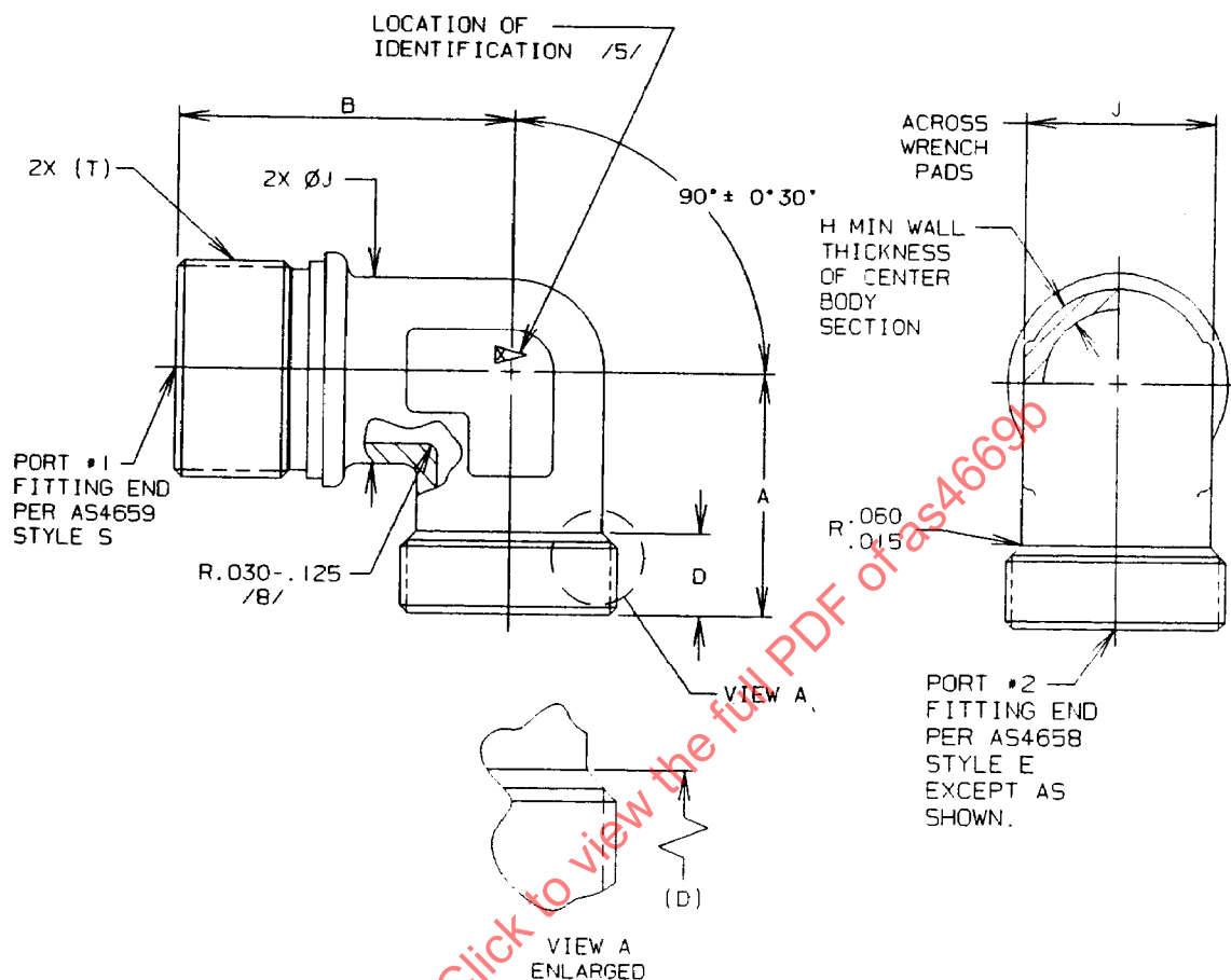
FIGURE 1 - FITTING, ELBOW, 90 DEGREE
