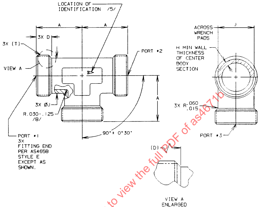
FIGURE 1 – FITTING, TEE
