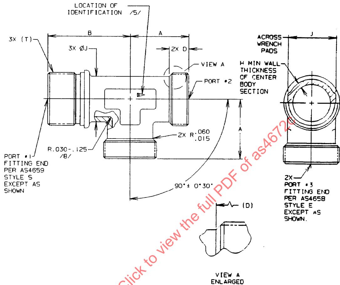
FIGURE 1 – FITTING, TEE
