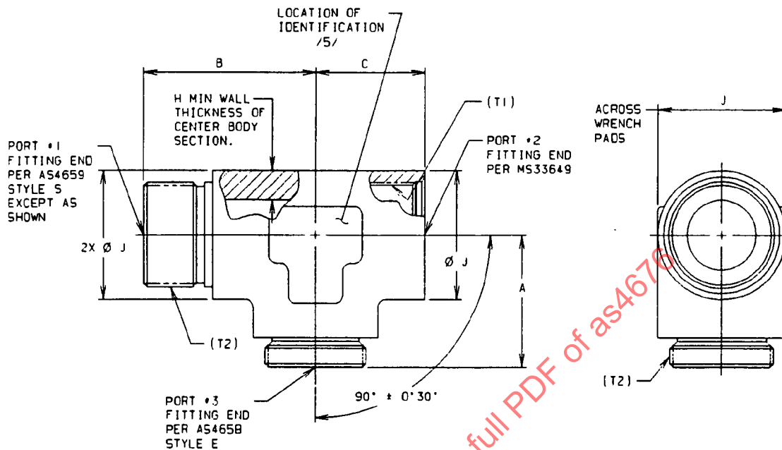
FIGURE 1 - TEE
