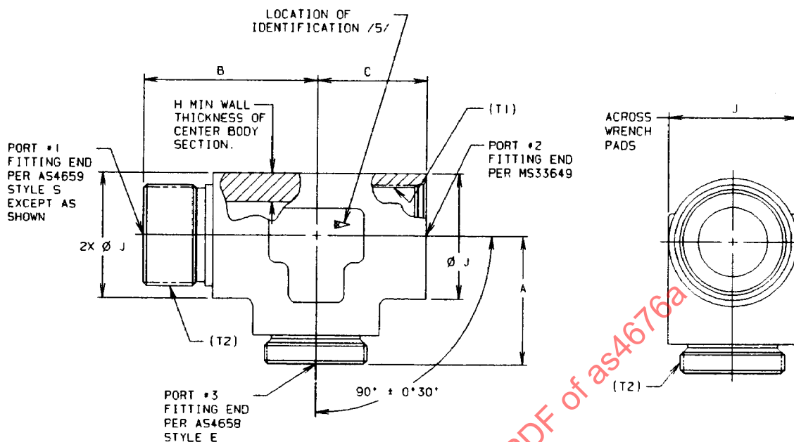
FIGURE 1 - FITTING, TEE
