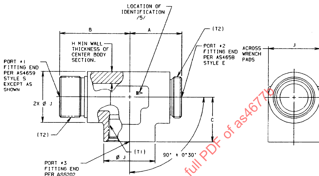
FIGURE 1 - FITTING, TEE
