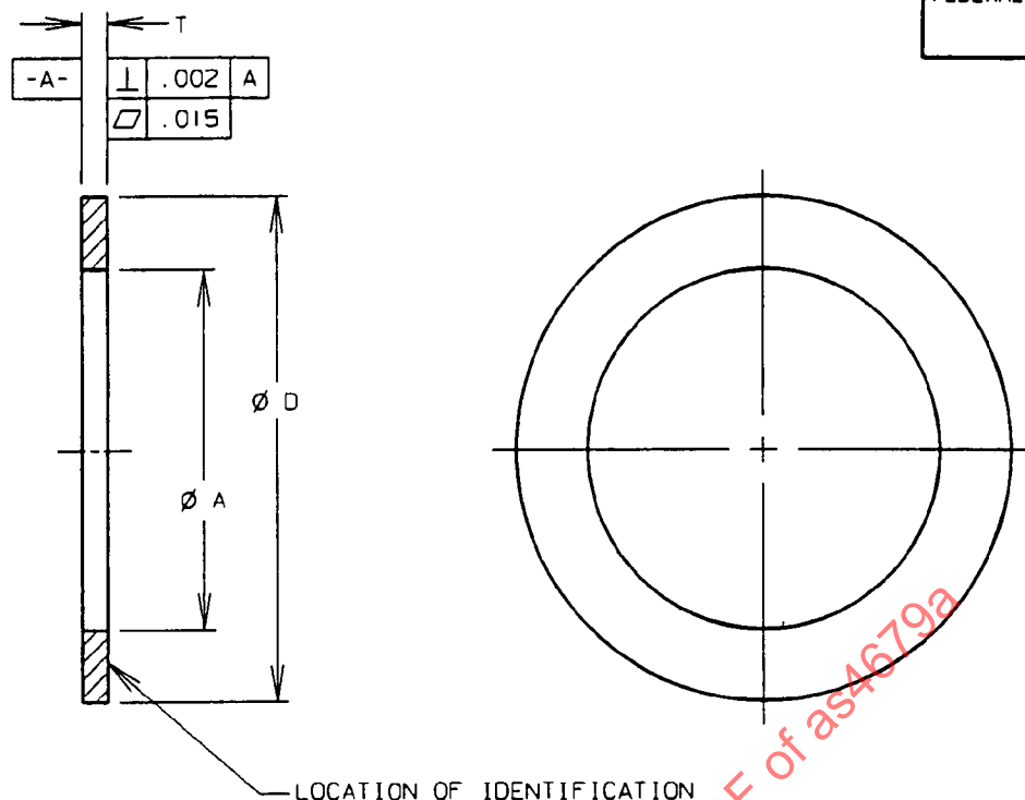
FIGURE 1 - WASHER
