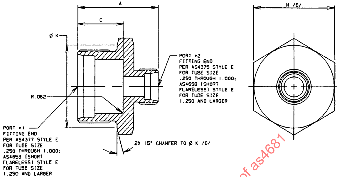
FIGURE 1 - UNION, REDUCER, BULKHEAD, FLARELESS END SHOWN AS REDUCER
