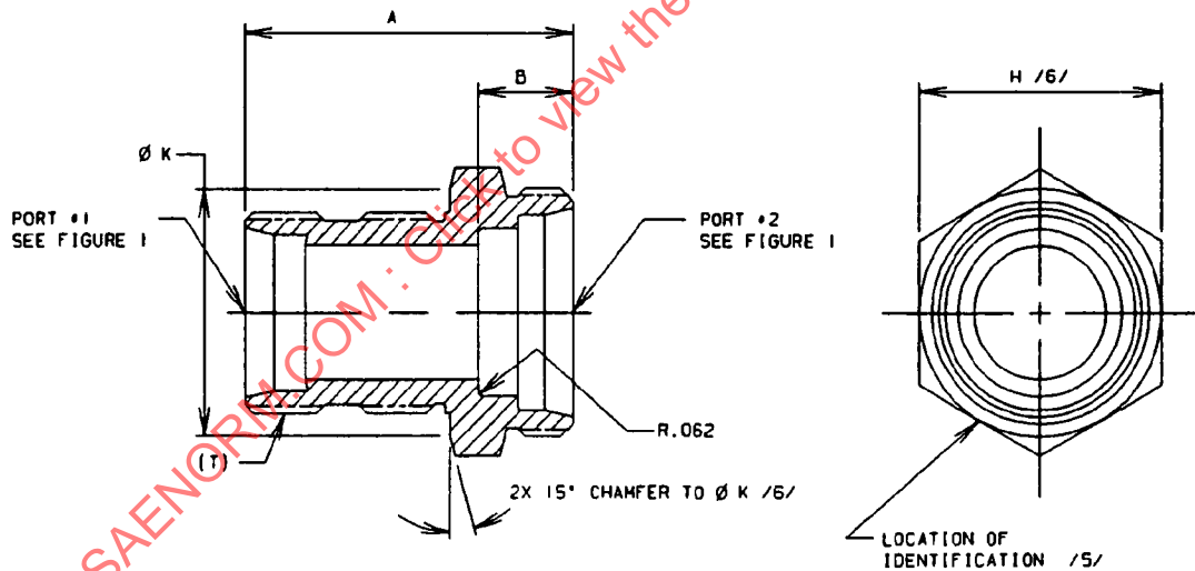
FIGURE 2 - UNION, EXPANDER, BULKHEAD, BULKHEAD END SHOWN AS REDUCER
