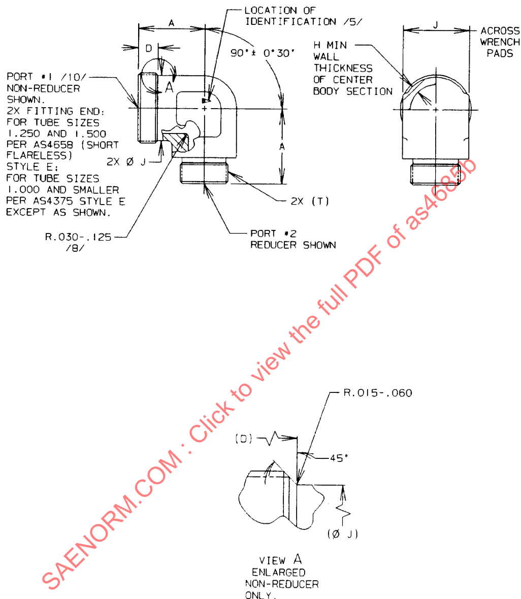
FIGURE 1 - FITTING, ELBOW, 90°, REDUCER
