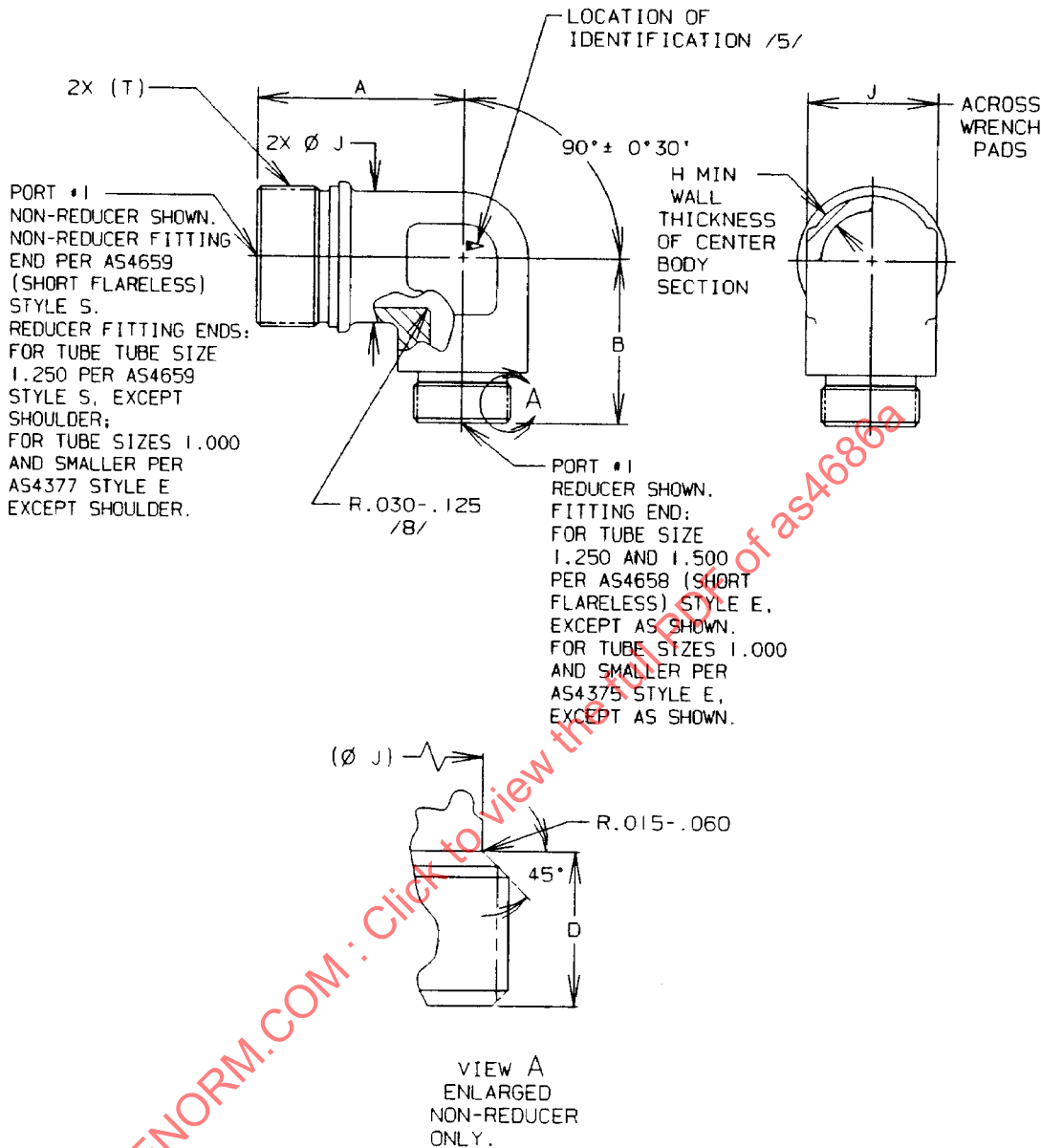
FIGURE 1 - FITTING, ELBOW, 90°, REDUCER
