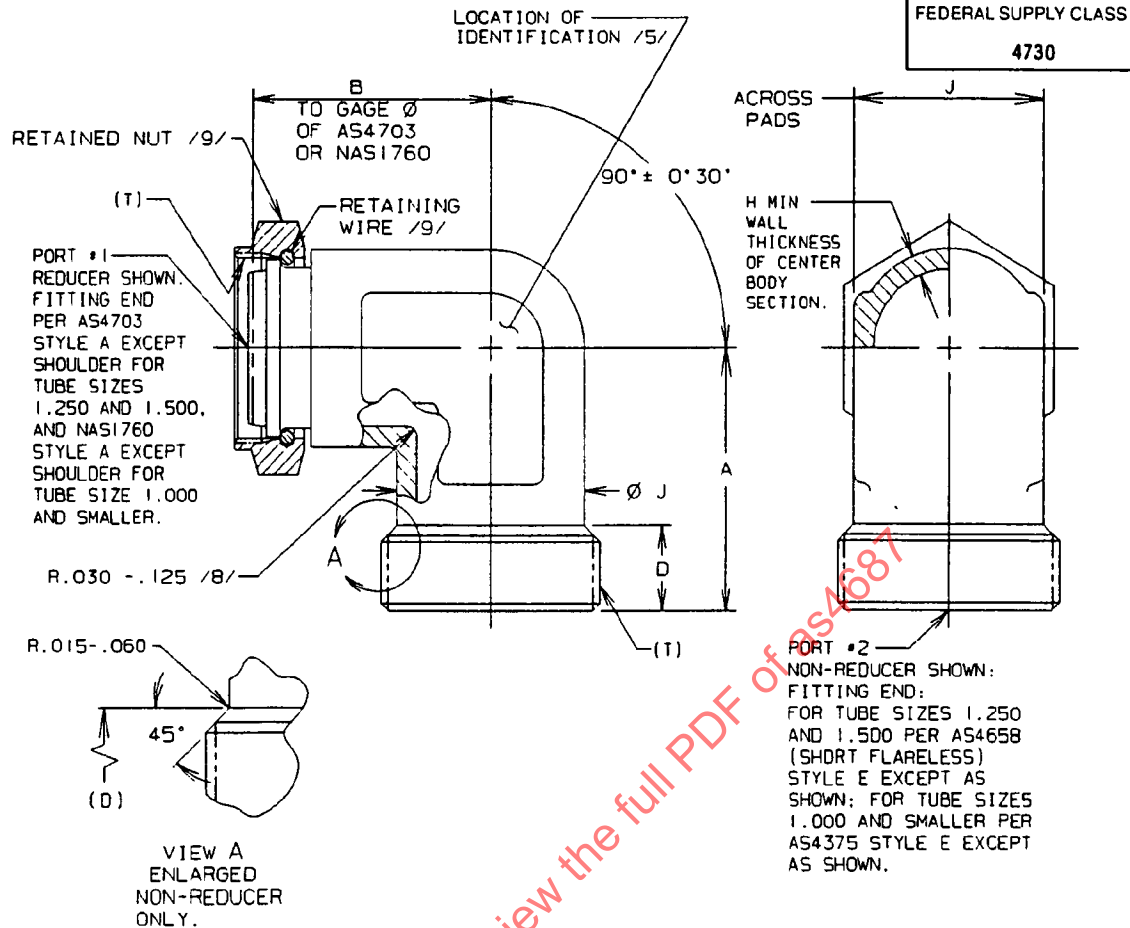
FIGURE 1 - ELBOW ASSEMBLY, 90°
