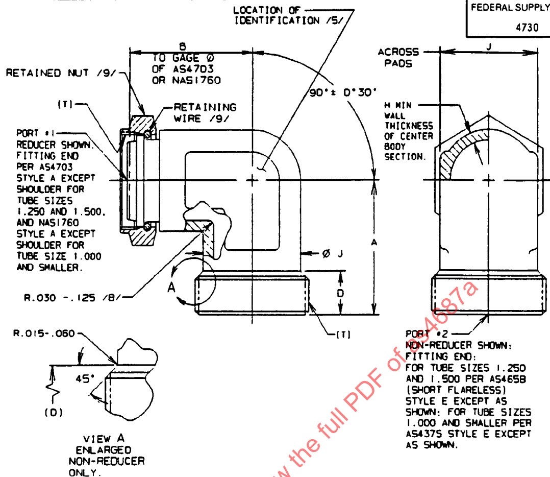
FIGURE 1 - ELBOW ASSEMBLY, 90°
