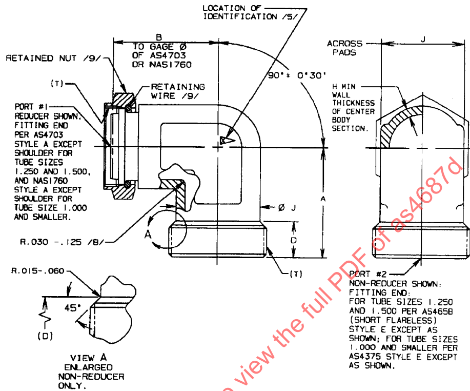
FIGURE 1 - ELBOW ASSEMBLY, 90°
