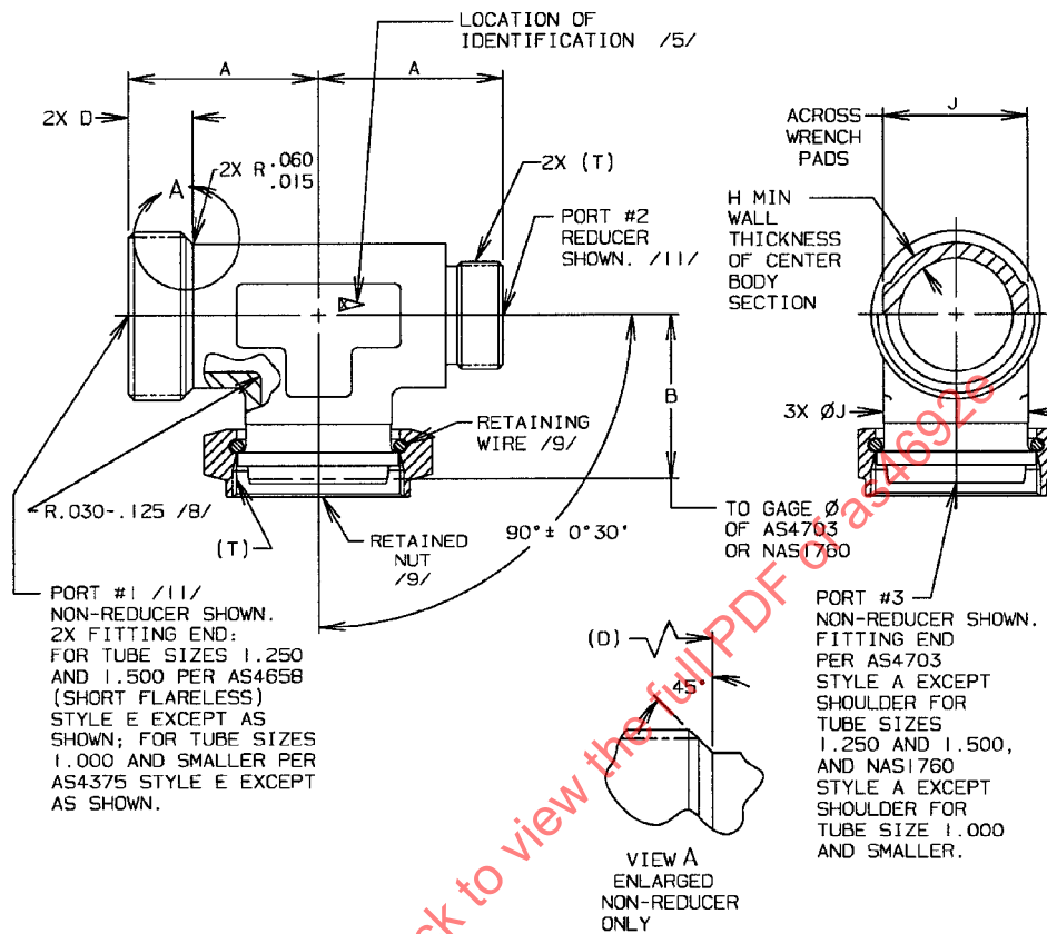
FIGURE 1 - TEE ASSEMBLY
