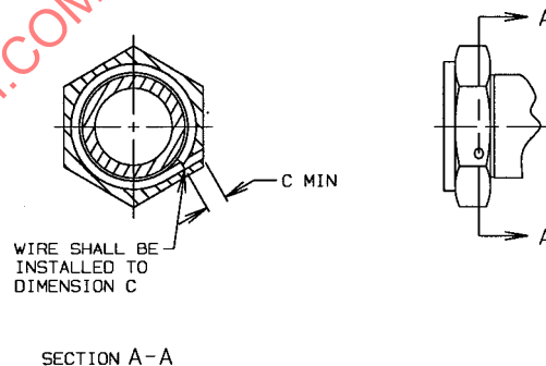
FIGURE 2 - INSTALLATION, RETAINED NUT AND RETAINING WIRE
