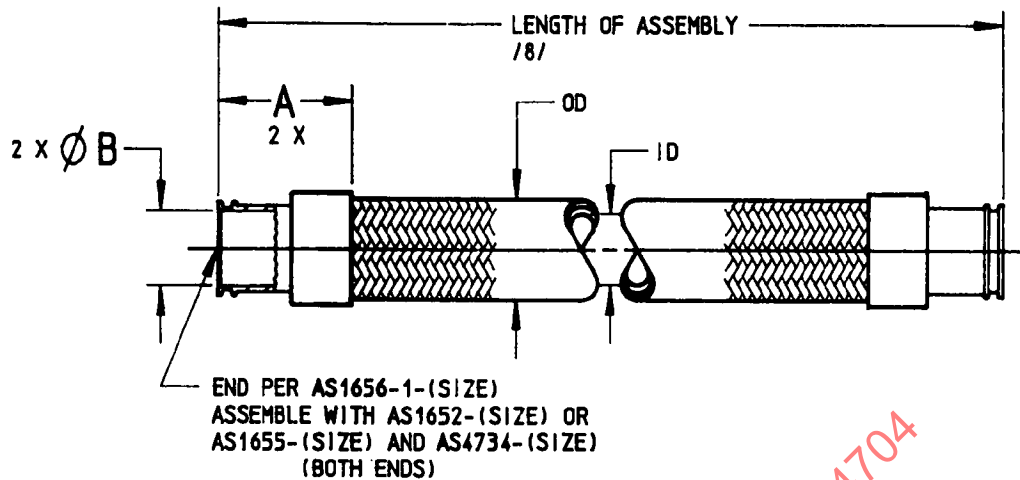
FIGURE 1 - HOSE ASSEMBLY
