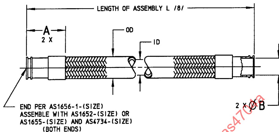
FIGURE 1 - HOSE ASSEMBLY
