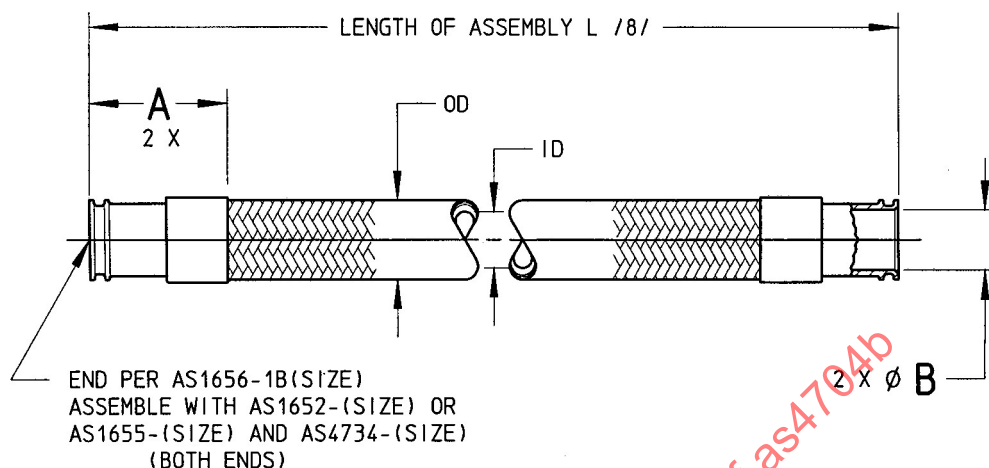
FIGURE 1 - HOSE ASSEMBLY
