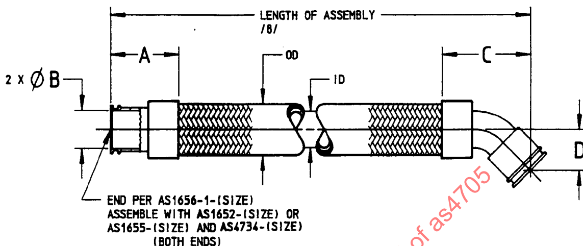
FIGURE 1 - HDSE ASSEMBLY
