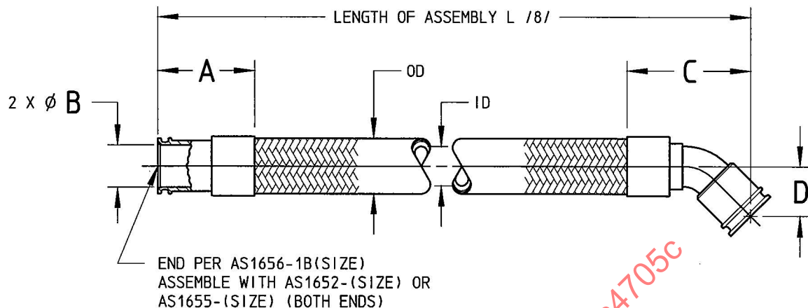
FIGURE 1 - HOSE ASSEMBLY
