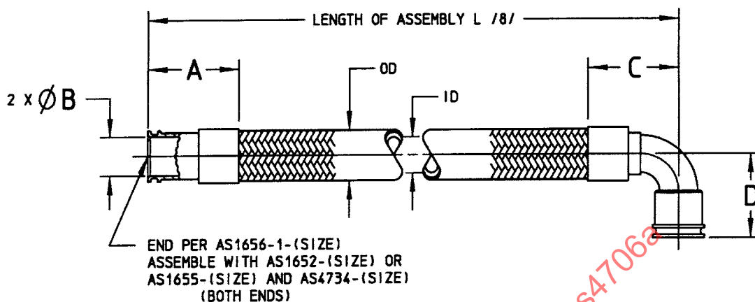
FIGURE 1 - HOSE ASSEMBLY
