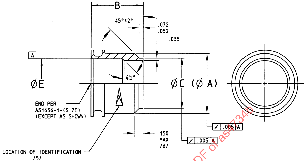
FIGURE 1 - MALE FERRULE
