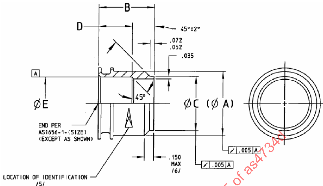
FIGURE 1 - MALE FERRULE
