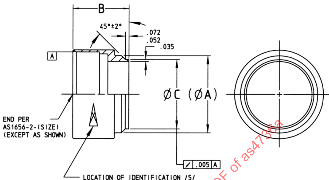
FIGURE 1 - FEMALE FERRULE
