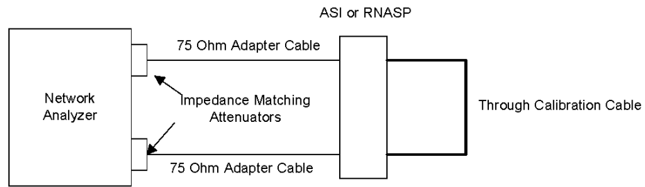
Equalization Loss Calibration - 75 Ohm
