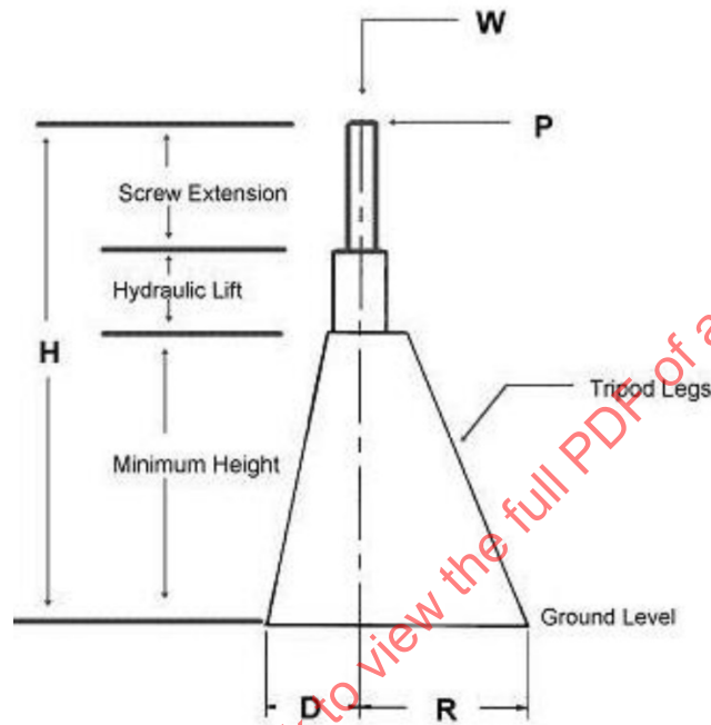
Figure 2 - Tripod leg design
