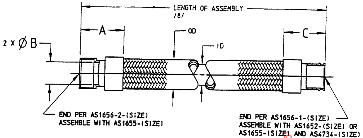
FIGURE 1 - HOSE ASSEMBLY
