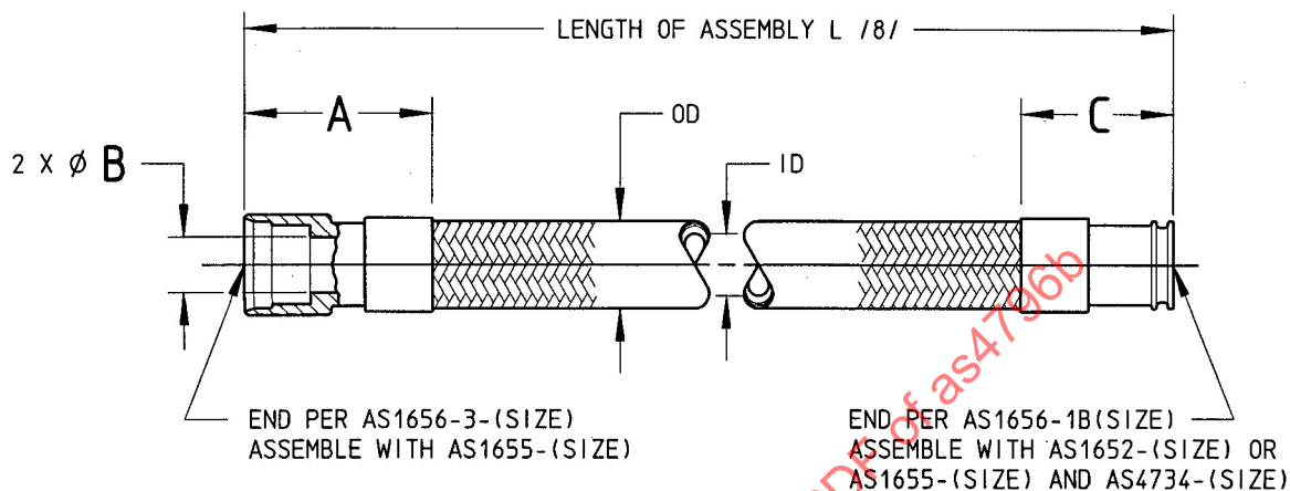
FIGURE 1 - HOSE ASSEMBLY
