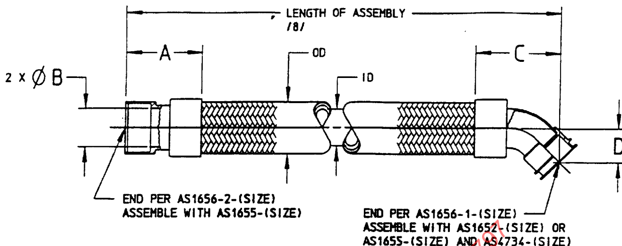
FIGURE 1 - HOSE ASSEMBLY
