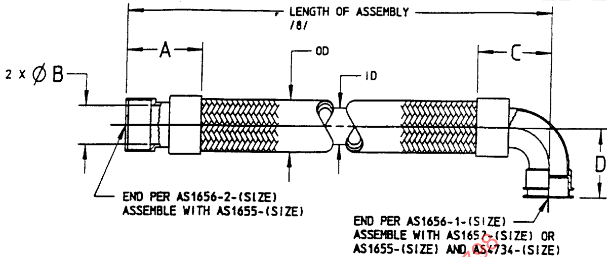
FIGURE 1 - HOSE ASSEMBLY
