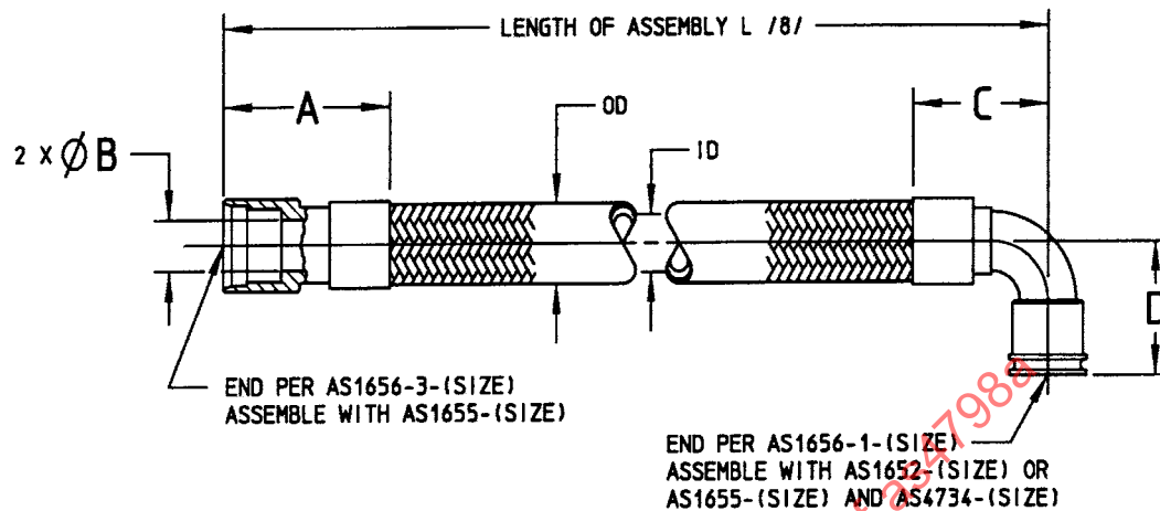
FIGURE 1 - HOSE ASSEMBLY
