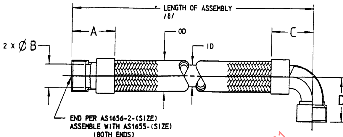
FIGURE 1 - HOSE ASSEMBLY
