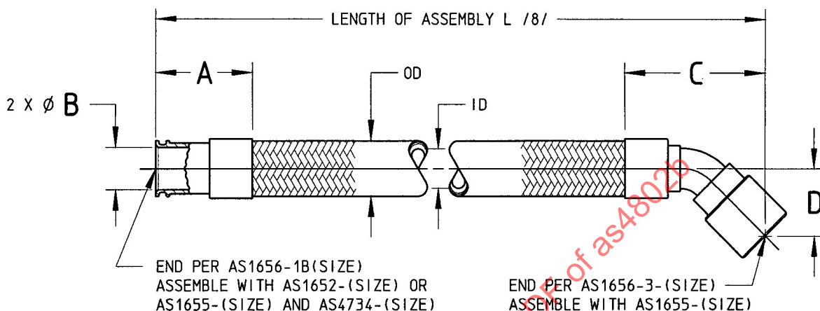
FIGURE 1 - HOSE ASSEMBLY
