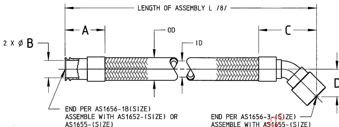
FIGURE 1 - HOSE ASSEMBLY
