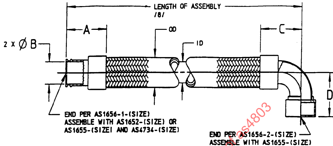
FIGURE 1 - HOSE ASSEMBLY
