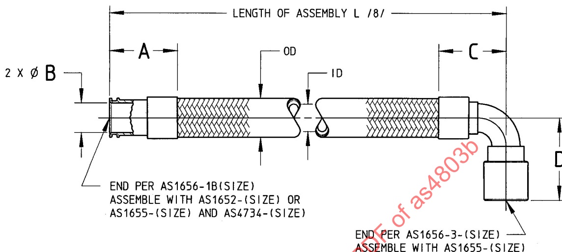
FIGURE 1 - HOSE ASSEMBLY
