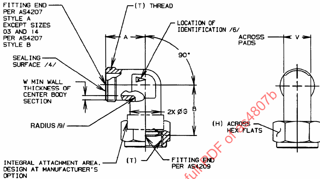
FIGURE 1 - FITTING ASSEMBLY, ELBOW, 90°
