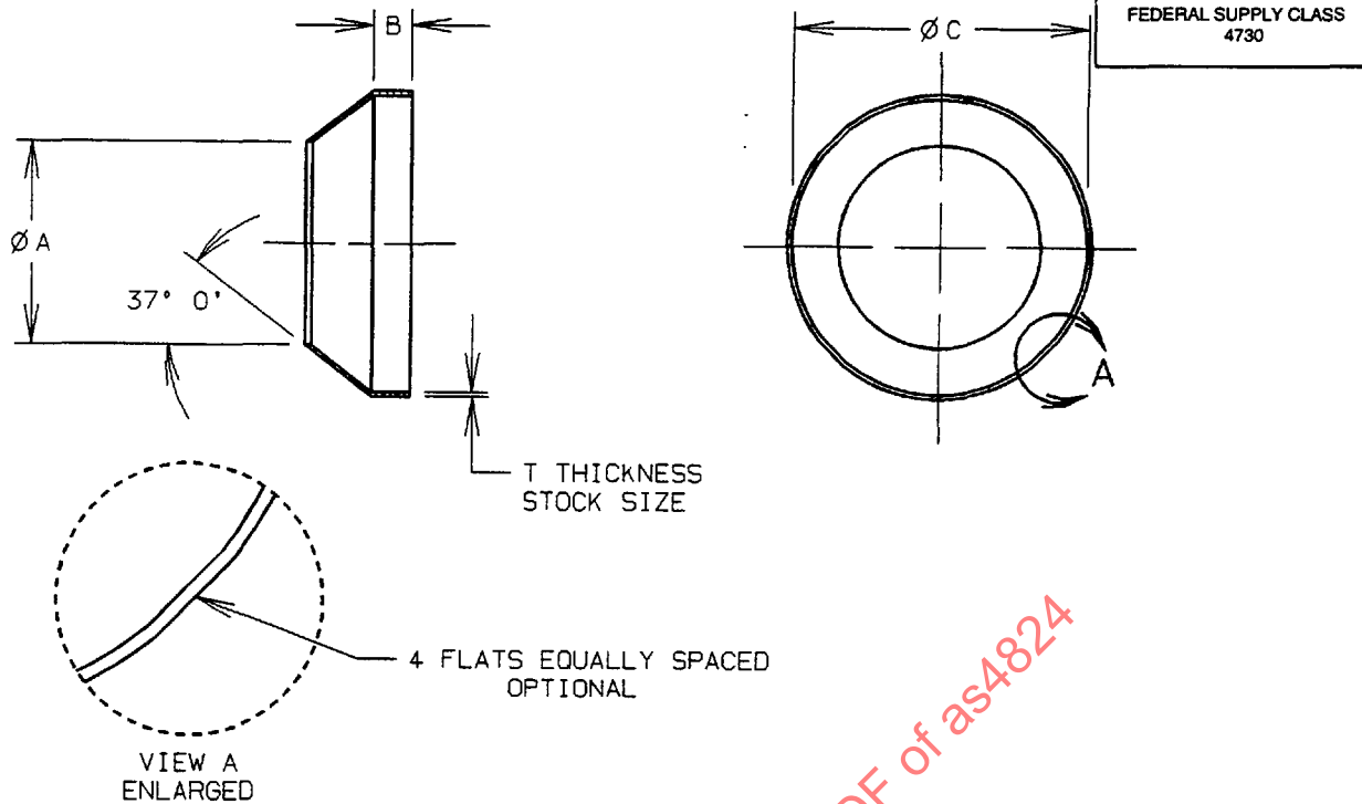
FIGURE 1 - GASKET
