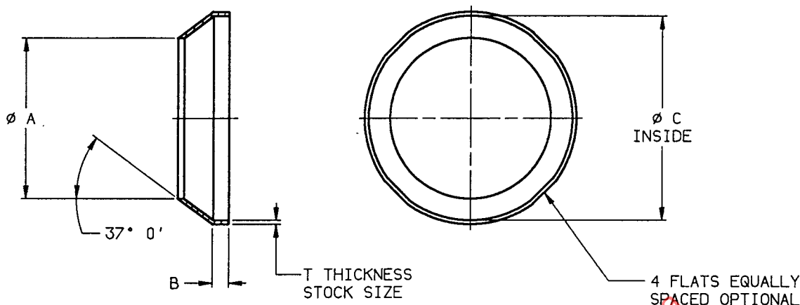
FIGURE 1 - GASKET
