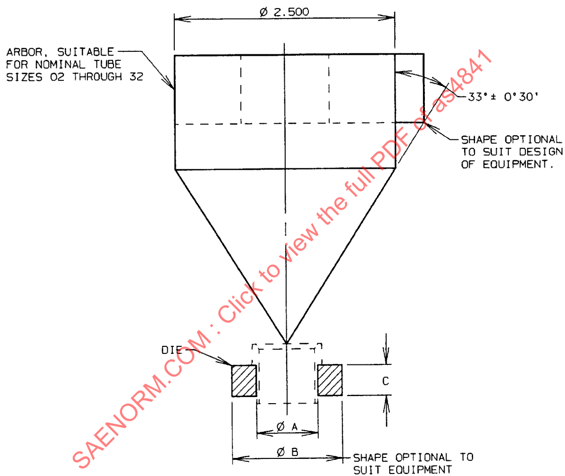
FIGURE 2 - Fixture for Testing Sleeves Dimensions in Inches, See Table 5
