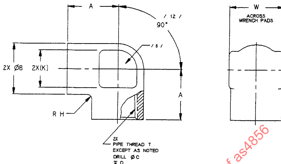
FIGURE 1 - ELBOW, 90°, PIPE, INTERNAL THREAD
