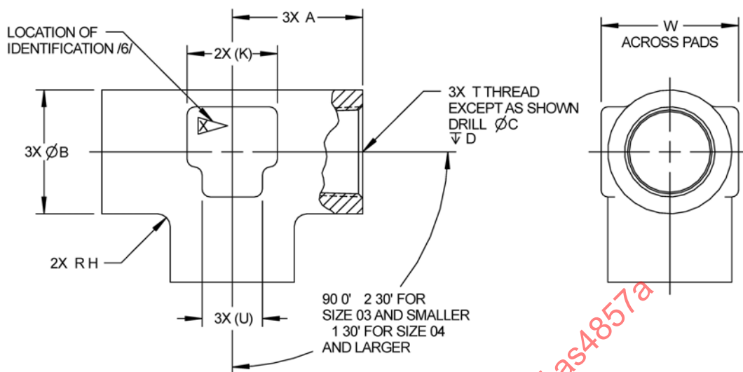
FIGURE 1 – FITTING, TEE, PIPE, INTERNAL THREAD
