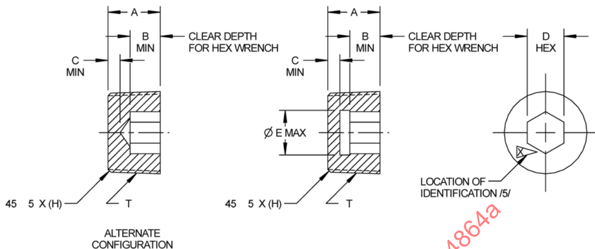
FIGURE 1 – FITTING, PLUG, PIPE, EXTERNAL THREAD, COUNTERSUNK HEX HEAD
