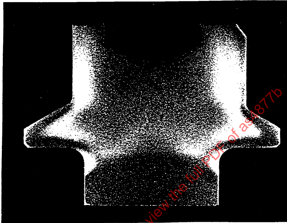
FIGURE 2B - Head-to-Shank Section Through Finished Part (Shows evidence that head was formed by forging.)
