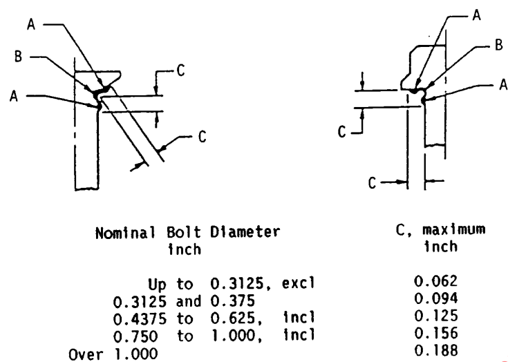
Figure 1 - Permissible distortion from fillet working
