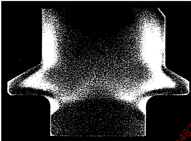
Figure 2B - Head-to-shank section through finished part (shows evidence that head was formed by forging)
